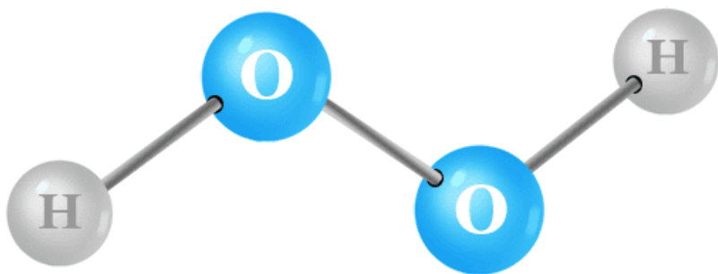
Hydrogen Peroxide ( H_2O_2 )
